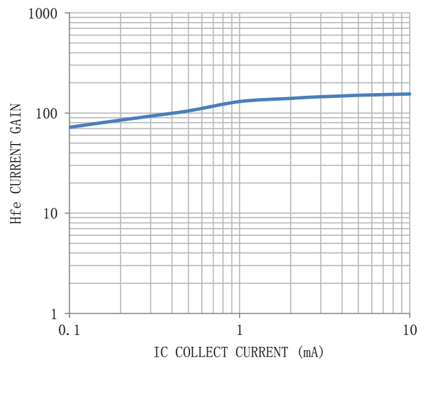
Figure 13. Current Gain
