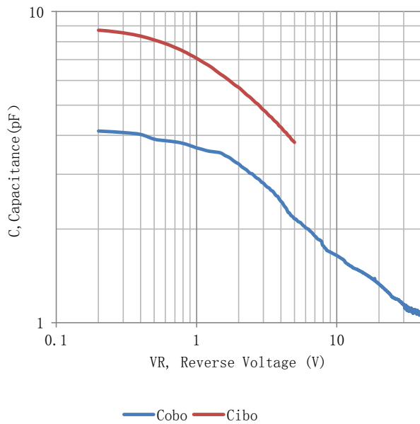
Figure 12. Capacitance
