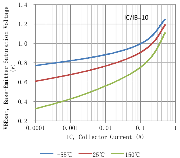
Figure 17. Base Emmitter Saturation Voltage vs. Collector
