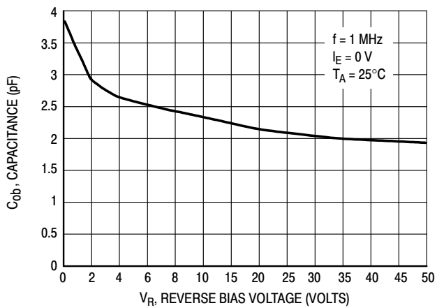
Figure 19. Output Capacitance
