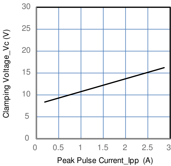
Fig5. Clamping Voltage vs. Peak Pulse Current
