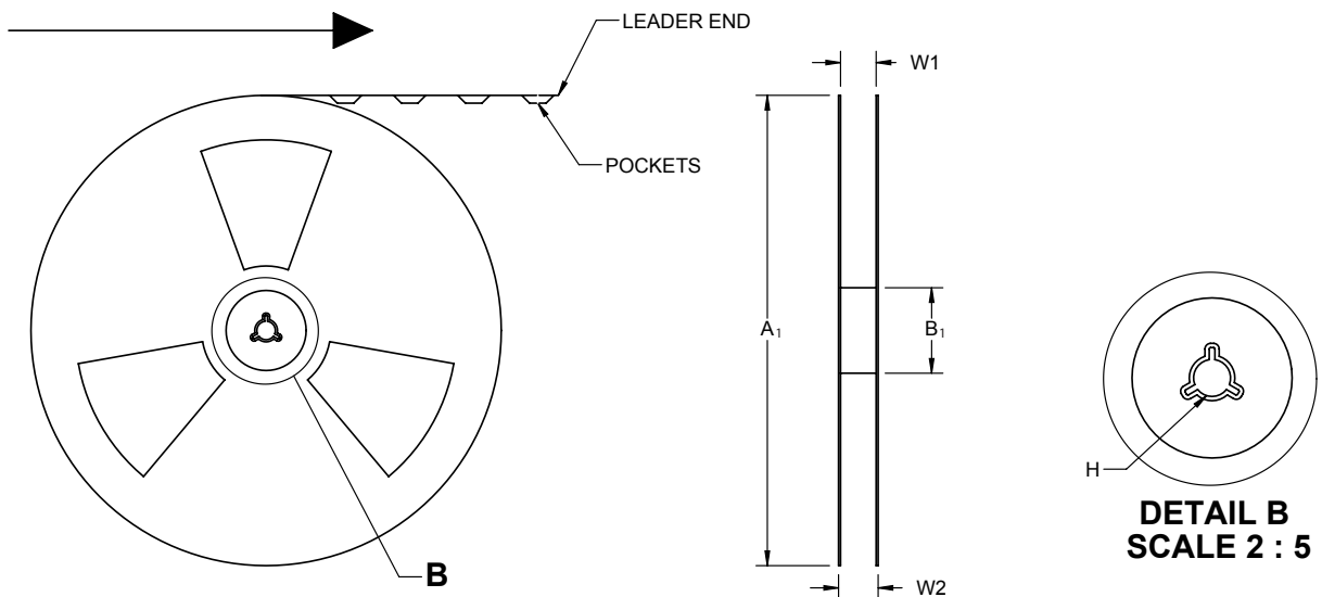
UNREELING DIRECTION
