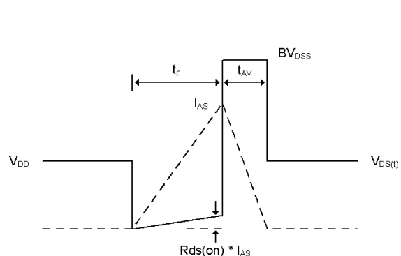
Fig18-2. Unclamped inductive waveform
