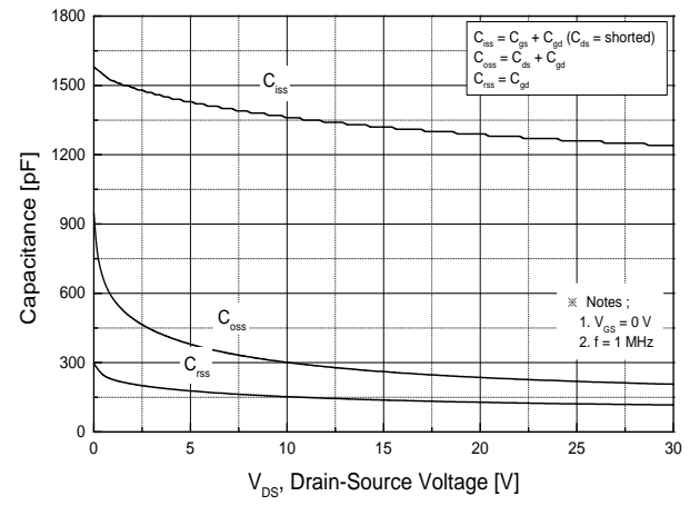
Fig.8 Capacitance Characteristics
