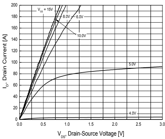
Fig.1 On-Region Characteristics
