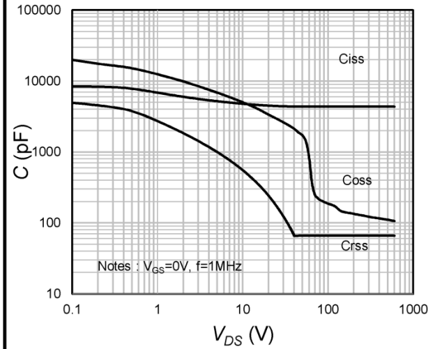
Fig.8 Capacitance Characteristics
