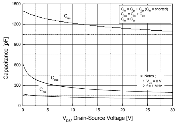
Fig.8 Capacitance Characteristics
