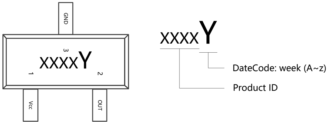
Figure.12 SOT-23 (Thin Outline) Chip Marking Spec
