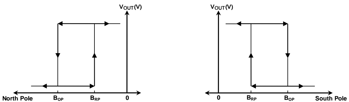
Switching Behavior
