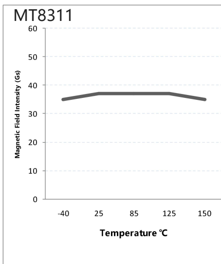
Figure.8 Magnetic Characteristics vs. Temperature (BHYST)
