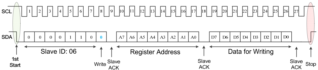
Figure 18: I 2 C Write
