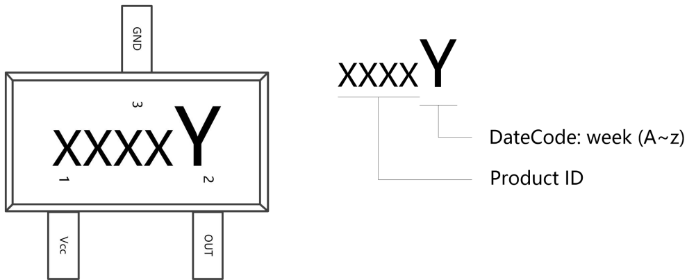
Figure.10 SOT-23-3L Chip Marking Spec
