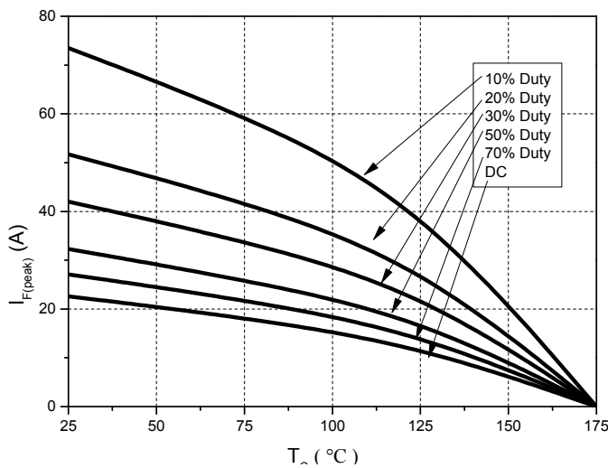
Figure 7. Current Derating
