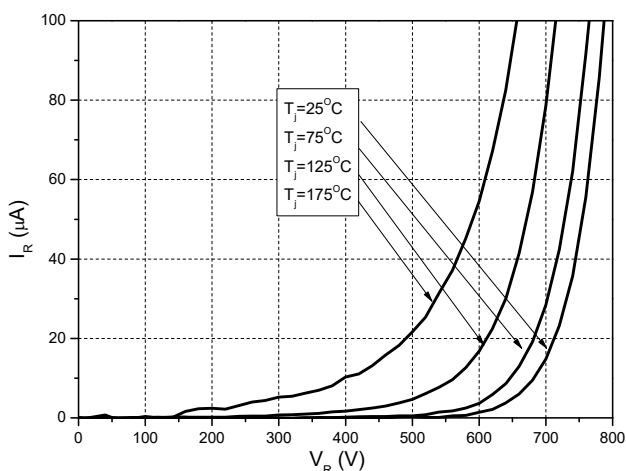
Figure 2. Reverse Characteristics
