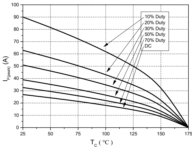
Figure 7. Current Derating
