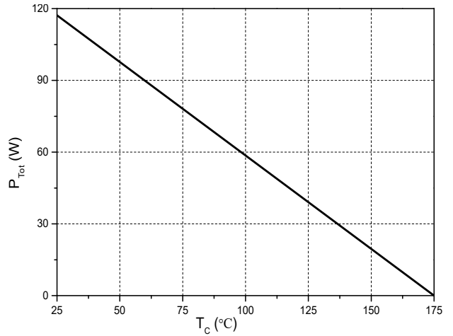
Figure 6. Power Derating
