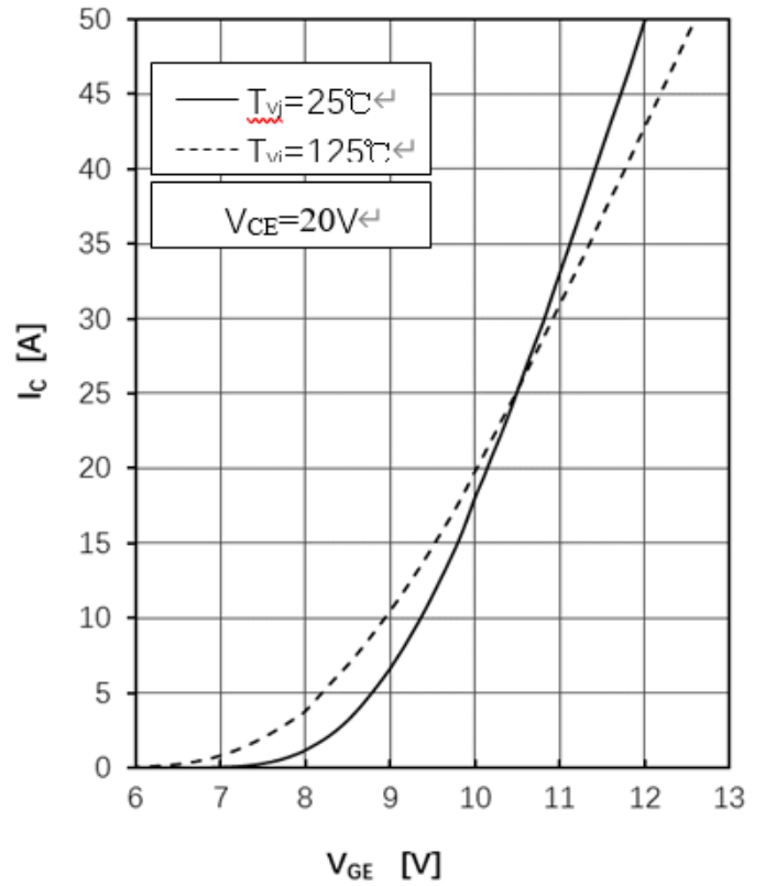
Fig2.IGBT Transfer Characteristics
