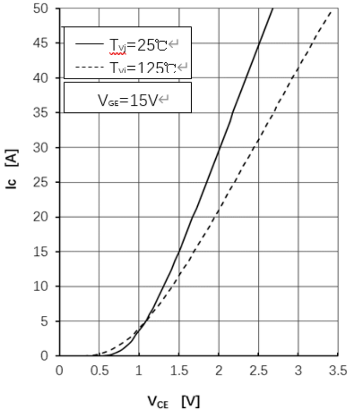
Fig1.IGBT Output Characteristics
