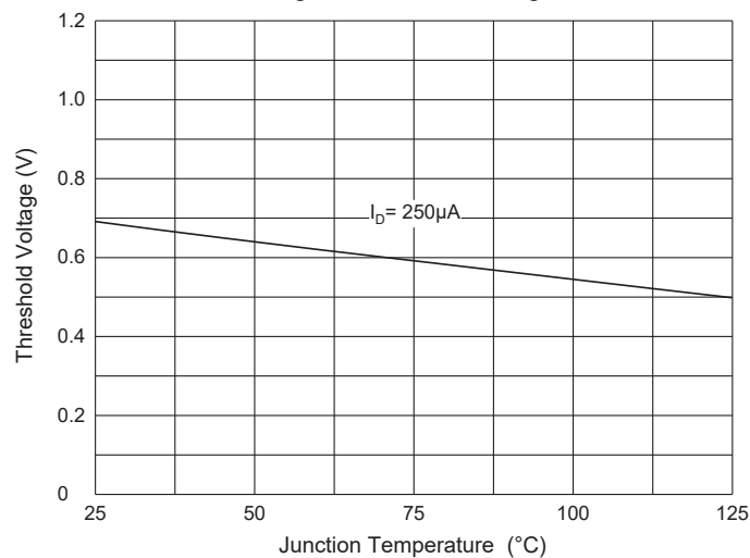
Fig. 6 - Threshold Voltage
