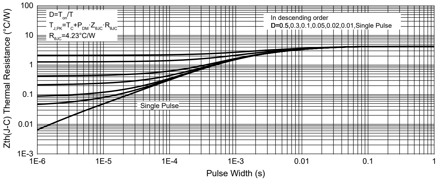
Fig. 7 - Maximum Transient Thermal Impedance
