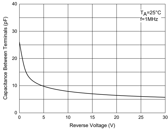
Fig. 4 - Capacitance Characteristics
