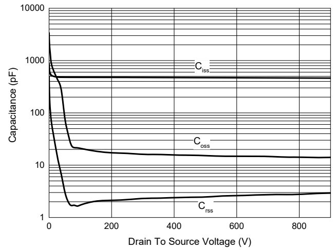
Fig. 8 - Capacitance Characteristics
