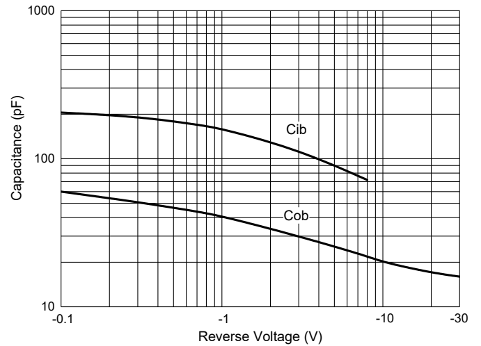
Fig. 6 - C_{ob}/C_{ib} - V_{CB}/V_{EB}
