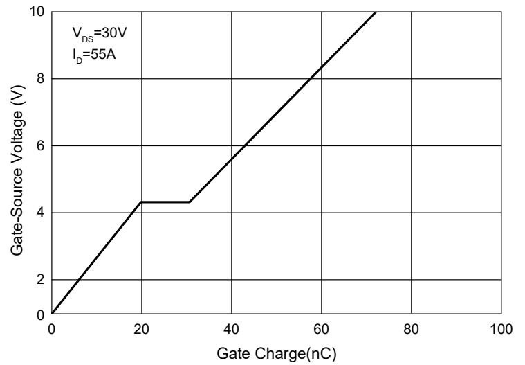
Fig. 8 - Gate Charge
