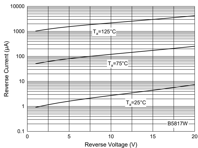
Fig. 3 - Reverse Characteristics
