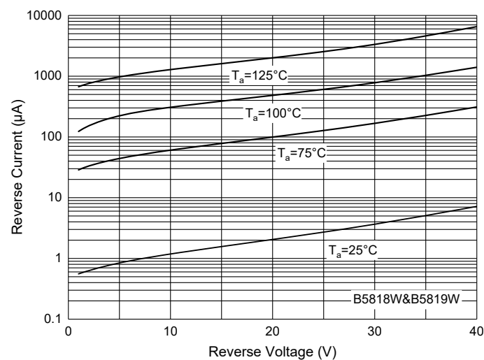
Fig. 4 - Reverse Characteristics
