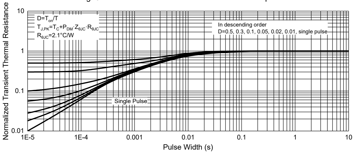
Fig. 8 - Normalized Maximum Transient Thermal Impedance
