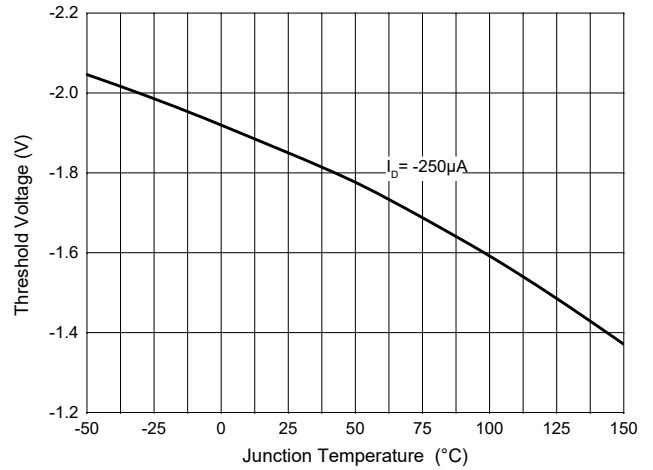
Fig. 6 - Threshold Voltage
