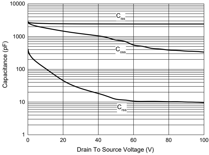
Fig. 7 - Capacitance Characteristics
