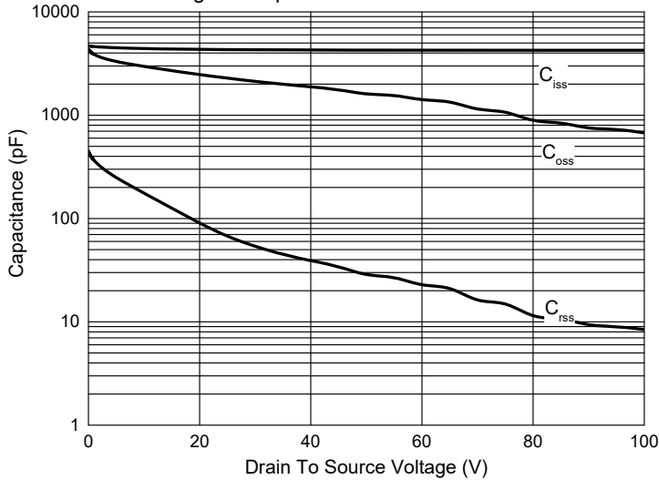
Fig. 5 - Capacitance Characteristics
