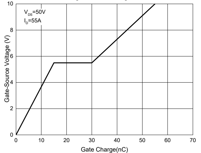
Fig. 6 - Gate Charge
