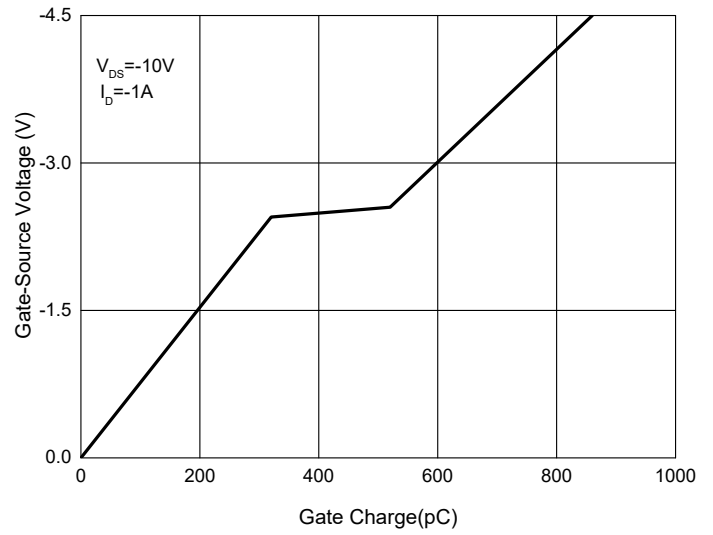
Fig. 8 - Gate Charge
