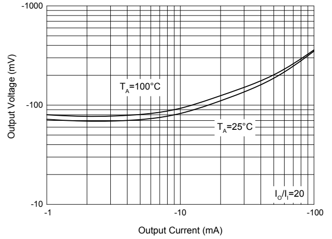
Fig. 4 - DTR2 Output Voltage Characteristics
