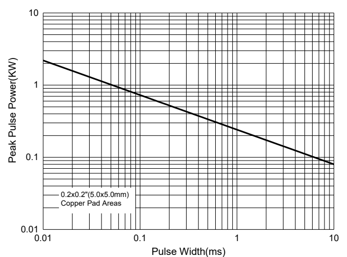
Fig. 6 - Non-Repetitive Peak Pulse Power
