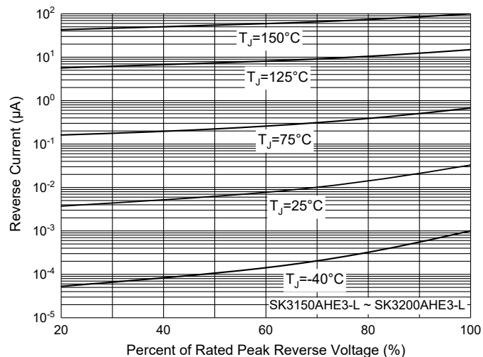
Fig. 10 - Typical Reverse Leakage Characteristics
