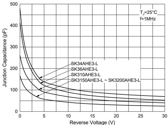
Fig. 11 - Capacitance Characteristics
