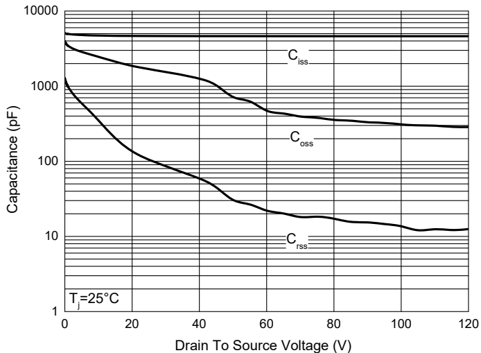
Fig. 7 - Capacitance Characteristics
