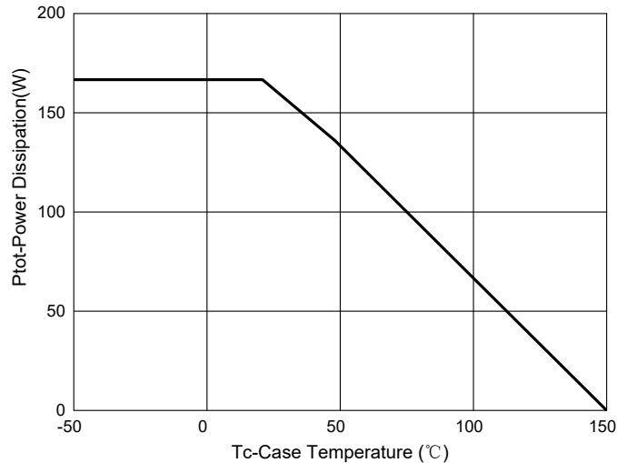
Fig. 8 - Power dissipation
