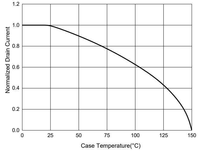
Fig. 8 - Normalized Drain Current Characteristics
