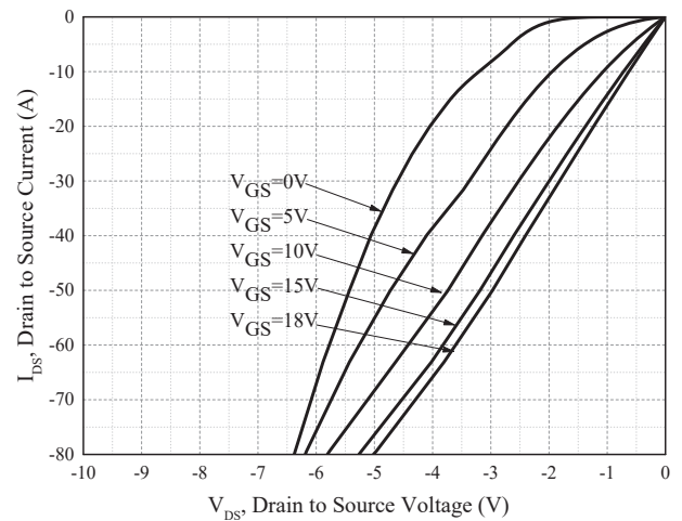
Fig. 10 - 3rd quadrant characteristic at T_j=25^\circ\text{C}
