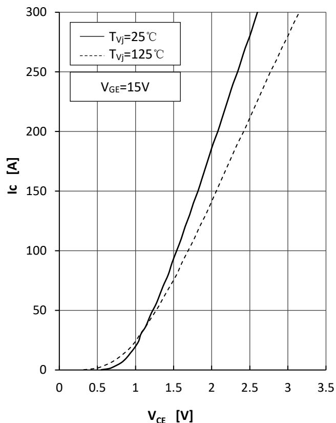
Fig1.IGBT Output Characteristics
