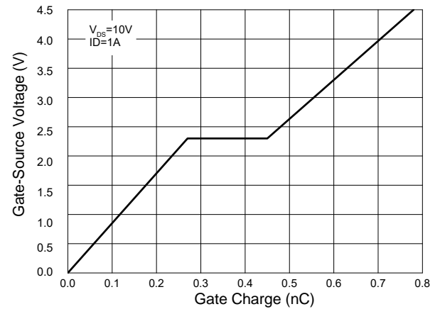
Fig.6 - Gate Charge
