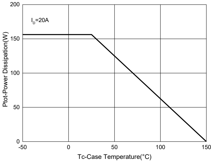
Fig. 9 - Power Dissipation
