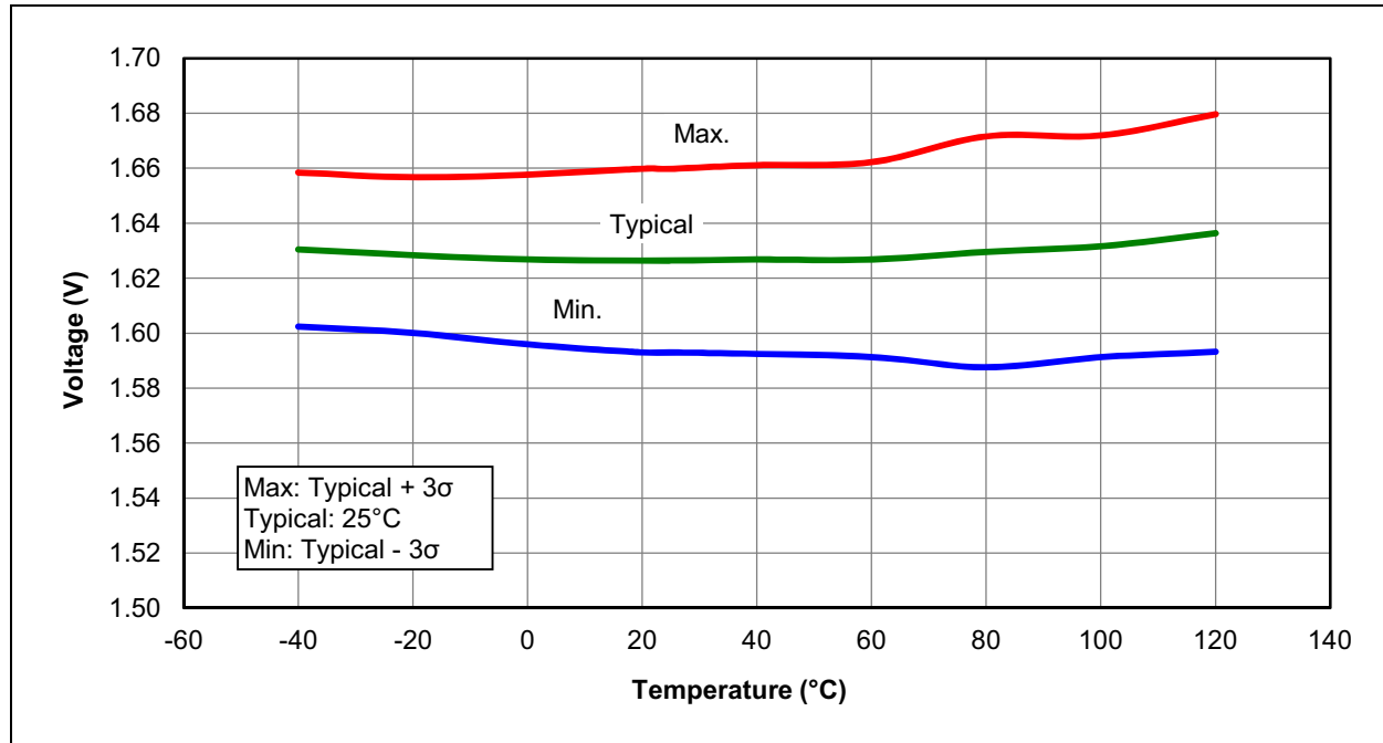
FIGURE 29-41: POR RELEASE VOLTAGE
