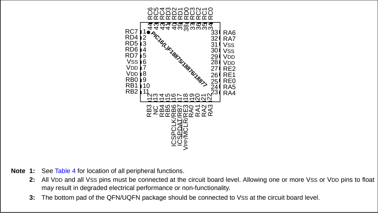
Pin Diagram – 44-Pin QFN (8x8)
