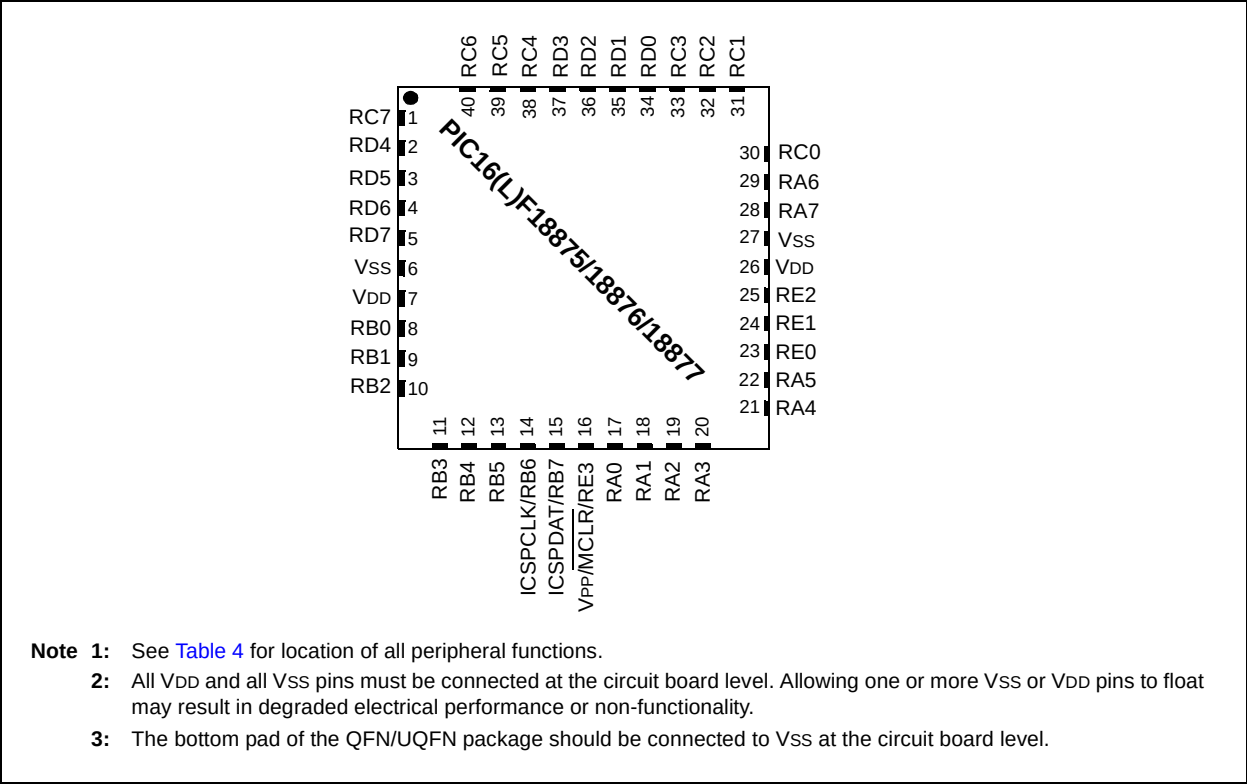
Pin Diagram – 40-Pin UQFN (5x5)
