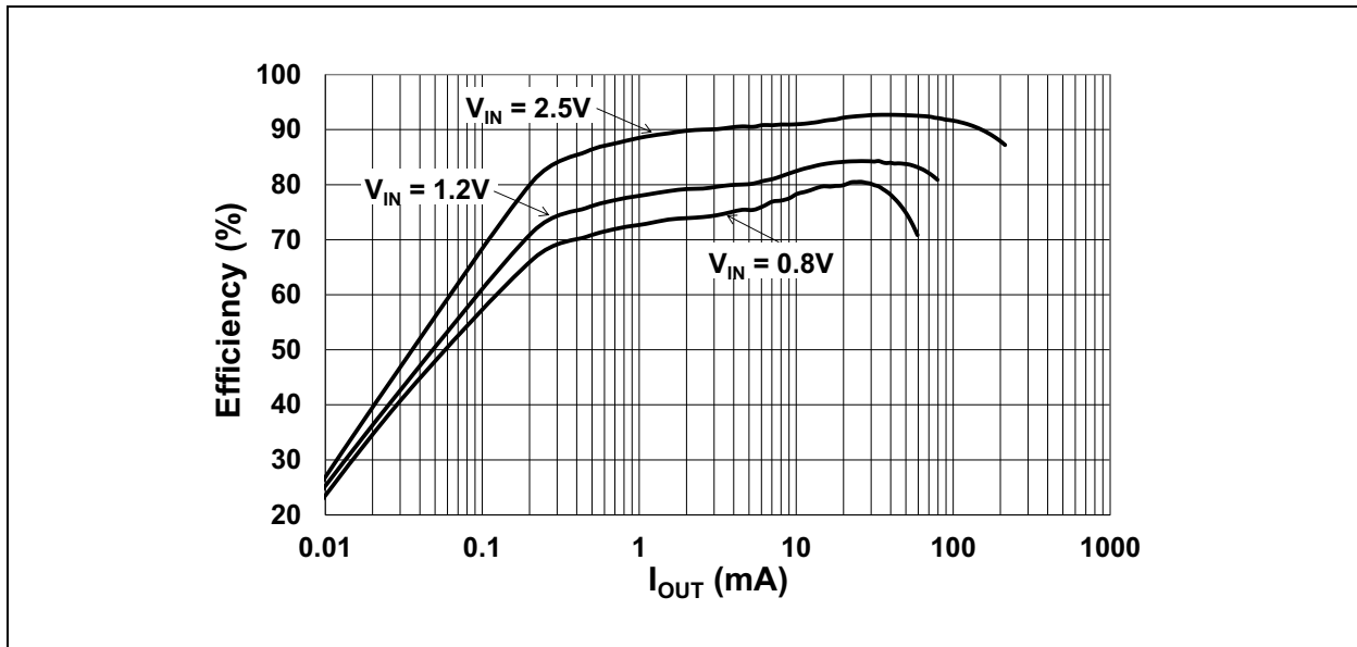
FIGURE 2: MCP1624 Efficiency vs. I_{OUT} , V_{OUT} = 3.3V .
