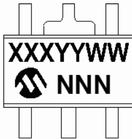
5-Lead SOT-89
