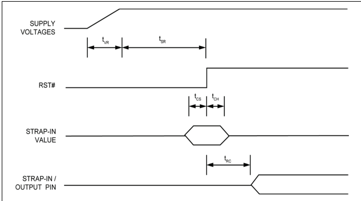
FIGURE 7-10: POWER-UP/RESET TIMING
