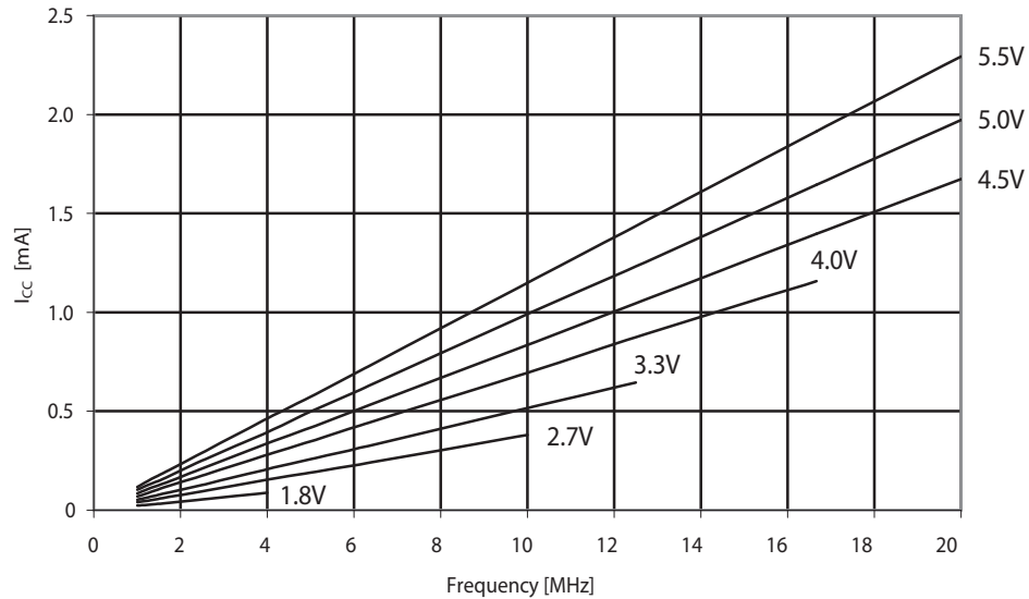
Figure 30-146. ATmega324A: Reset supply current vs. frequency (1 - 20MHz)
