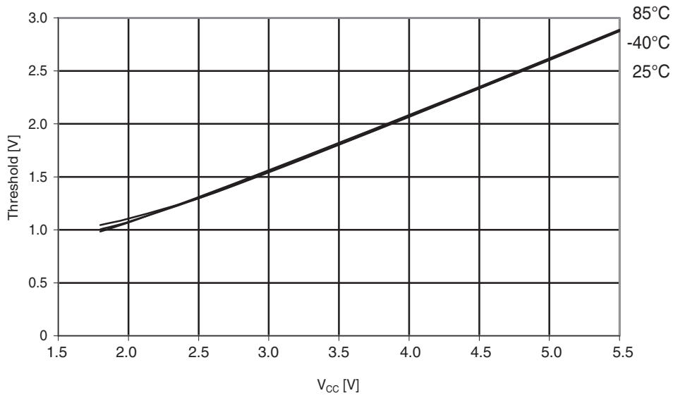
Figure 30-172. ATmega324PA: I/O pin input threshold vs. V_{CC} ( V_{IH} , I/O pin read as '1')
