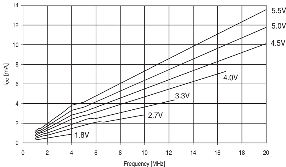
Figure 30-247. ATmega644PA: Active supply current vs. frequency (1 - 20MHz)
