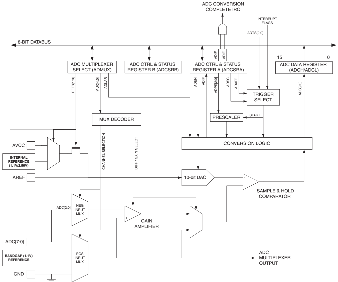
Figure 23-1. Analog-to-digital Converter block schematic
