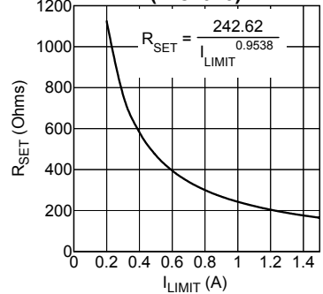
R SET vs. I LIMIT (MIC20X9)
