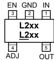
SOT-23-5 (Adjustable)
