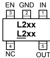
SOT-23-5 (Fixed)
