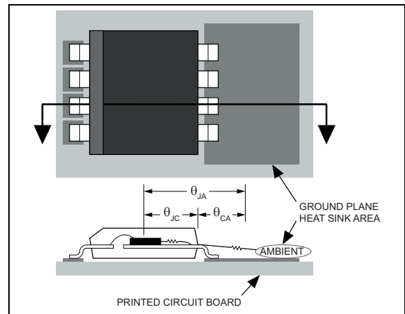
FIGURE 4-3: Thermal Resistance.
