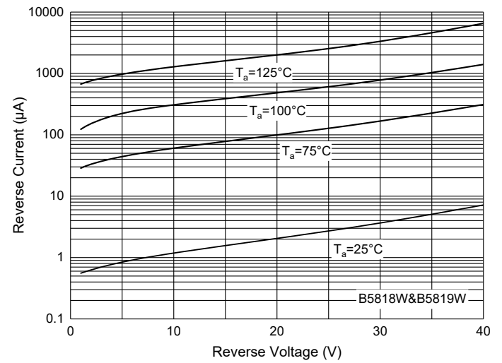
Fig. 4 - Reverse Characteristics
