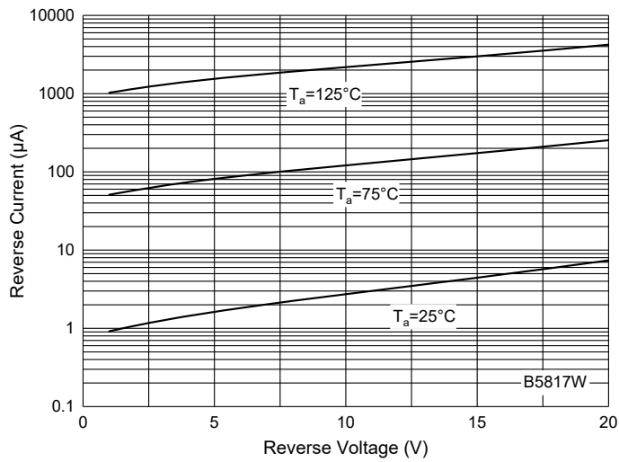
Fig. 3 - Reverse Characteristics
