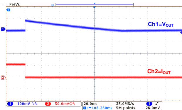
Load Transient: MD8333-1( I_{OUT}=50mA\sim 0mA )
