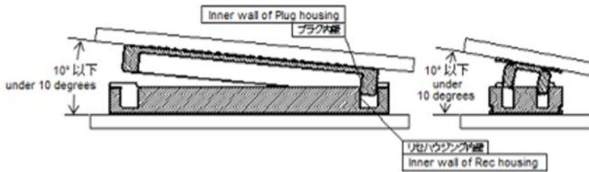
△ 図-2 内壁合せによる挿抜 (Acceptable) Figure-2 Mating aligning to inner wall of housings (Acceptable)
